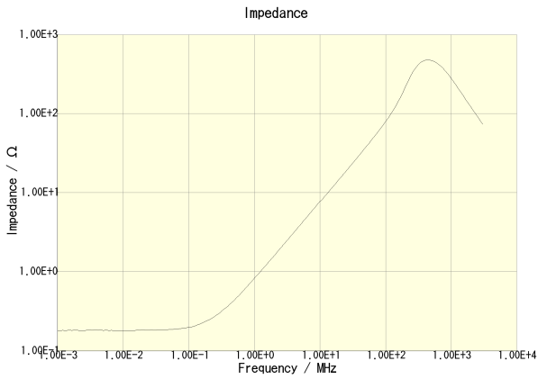
MLF1608DR12KTA00
