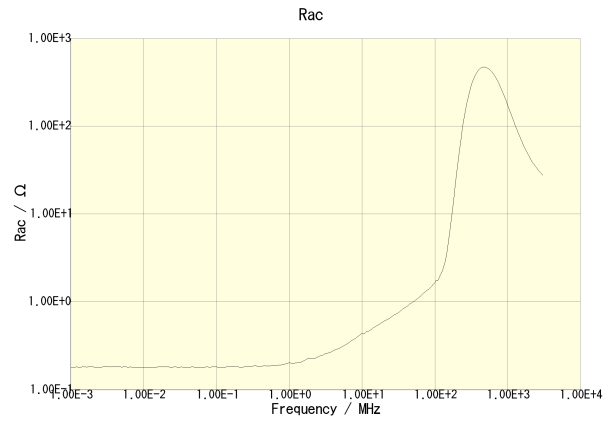
MLF1608DR12KTA00
