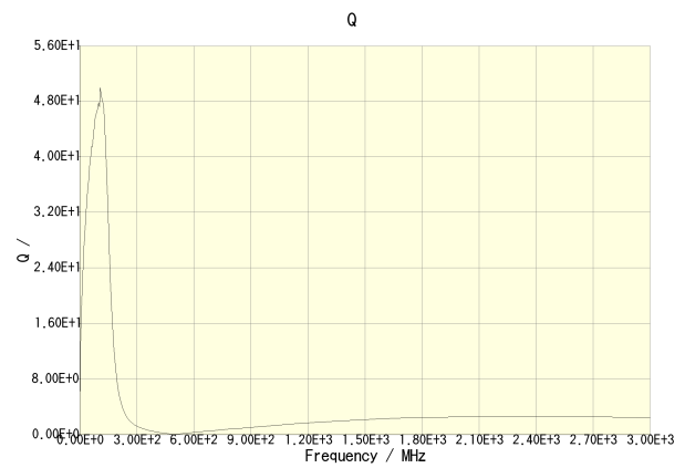
MLF1608DR12KTA00
